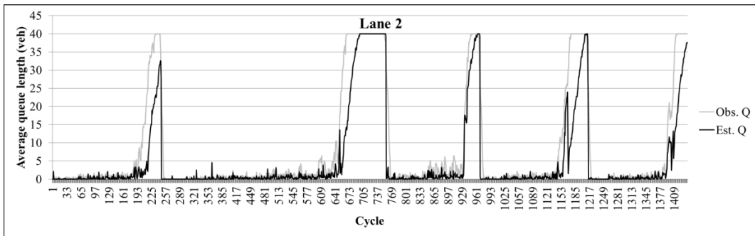
Fig. 3 (b). Comparison of average queue lengths as observed and estimated by Model III on lane 2.
