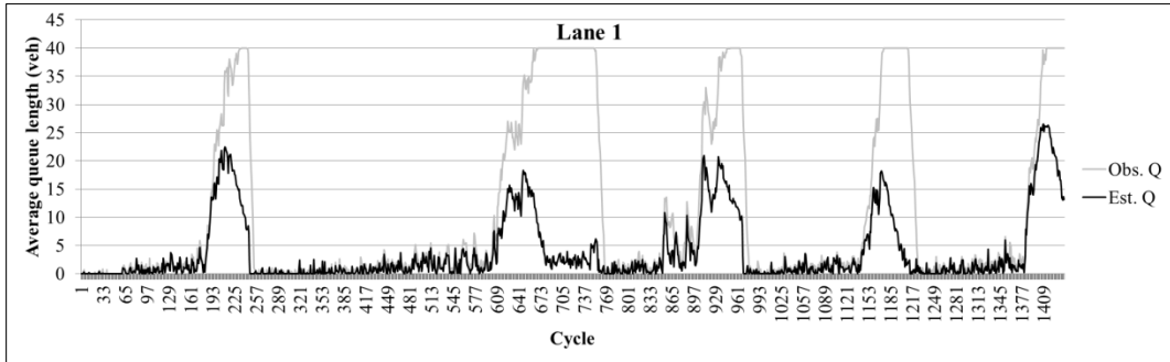
Fig. 3 (a). Comparison of average queue lengths as observed and estimated by Model III on lane 1.
