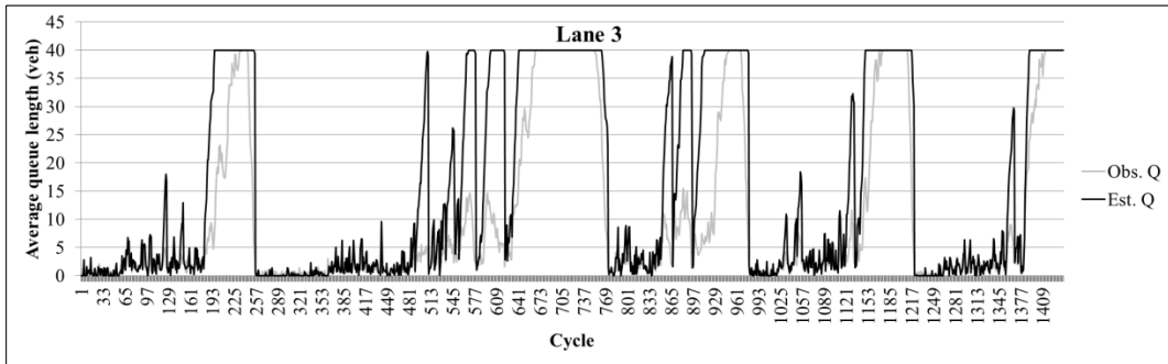
Fig. 3 (c). Comparison of average queue lengths as observed and estimated by Model III on lane 3.
