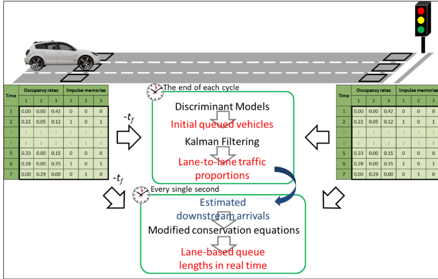
Fig. 1. Data-processing method for the deep learning approach to dynamic queue estimation.
