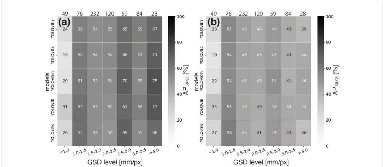
FIGURE 3 Detection performance dependence of OD (A) and IS (B) on the image resolution. The values above each panel denote the number of images at each resolution. The value in each box is the percentage of AP 50-95 , and the color scale is shown on the right side of each panel.
